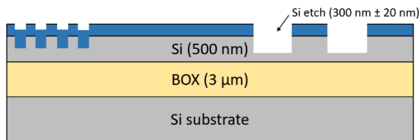
Grating Coupler
