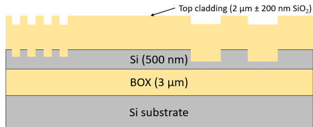
Grating Coupler
