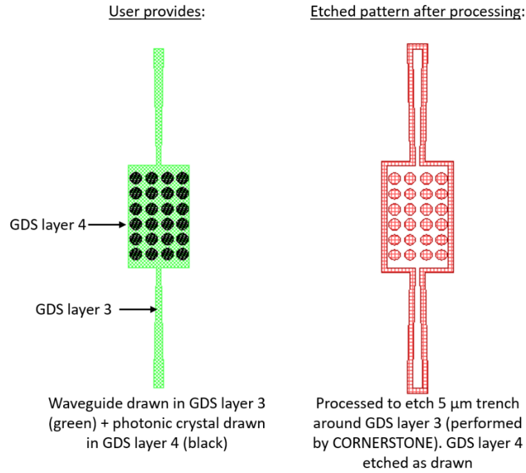
Figure 2 – Example photonic crystal structure using GDS Layers 3 & 4.
