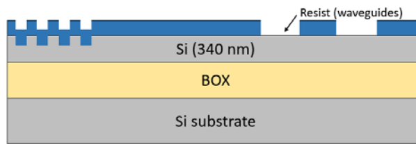
Grating Coupler
