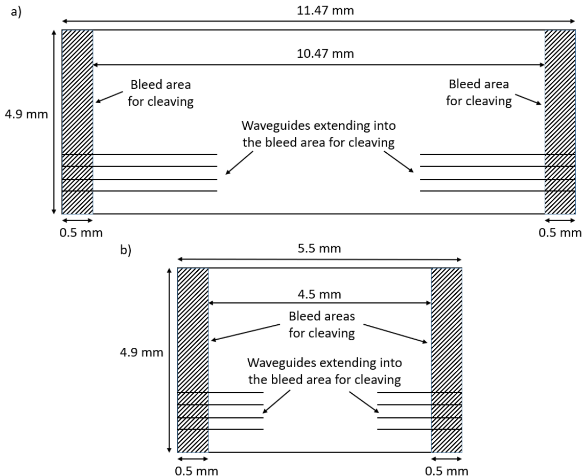
Figure 1 – User cell design area layout for a) 11.47 \times 4.9 \text{ mm}^2 , and b) 5.5 \times 4.9 \text{ mm}^2 .
