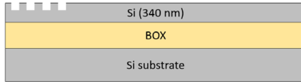
Grating Coupler
