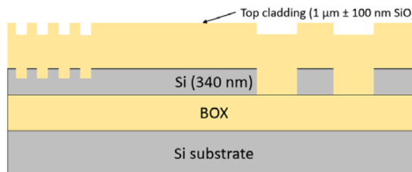
Grating Coupler
