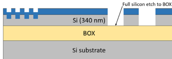
Grating Coupler
