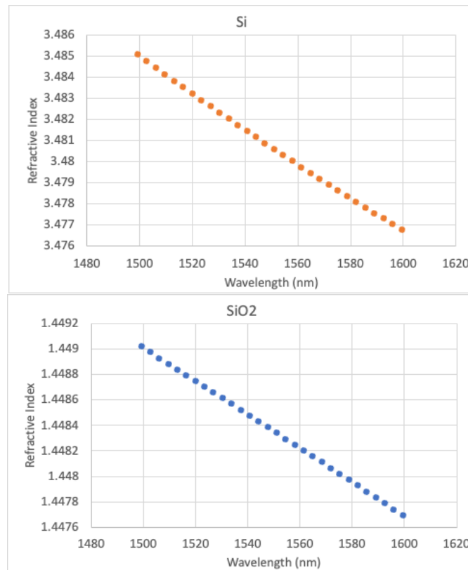
Figure 4 – Refractive indices of Silicon(upper) and \text{SiO}_2 (bottom).
